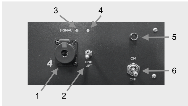
Figure 2. 4DI Front Panel Controls and Connections
